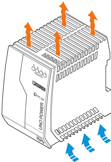
Figure 3 Convection
